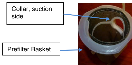
Filter assembly – top view
